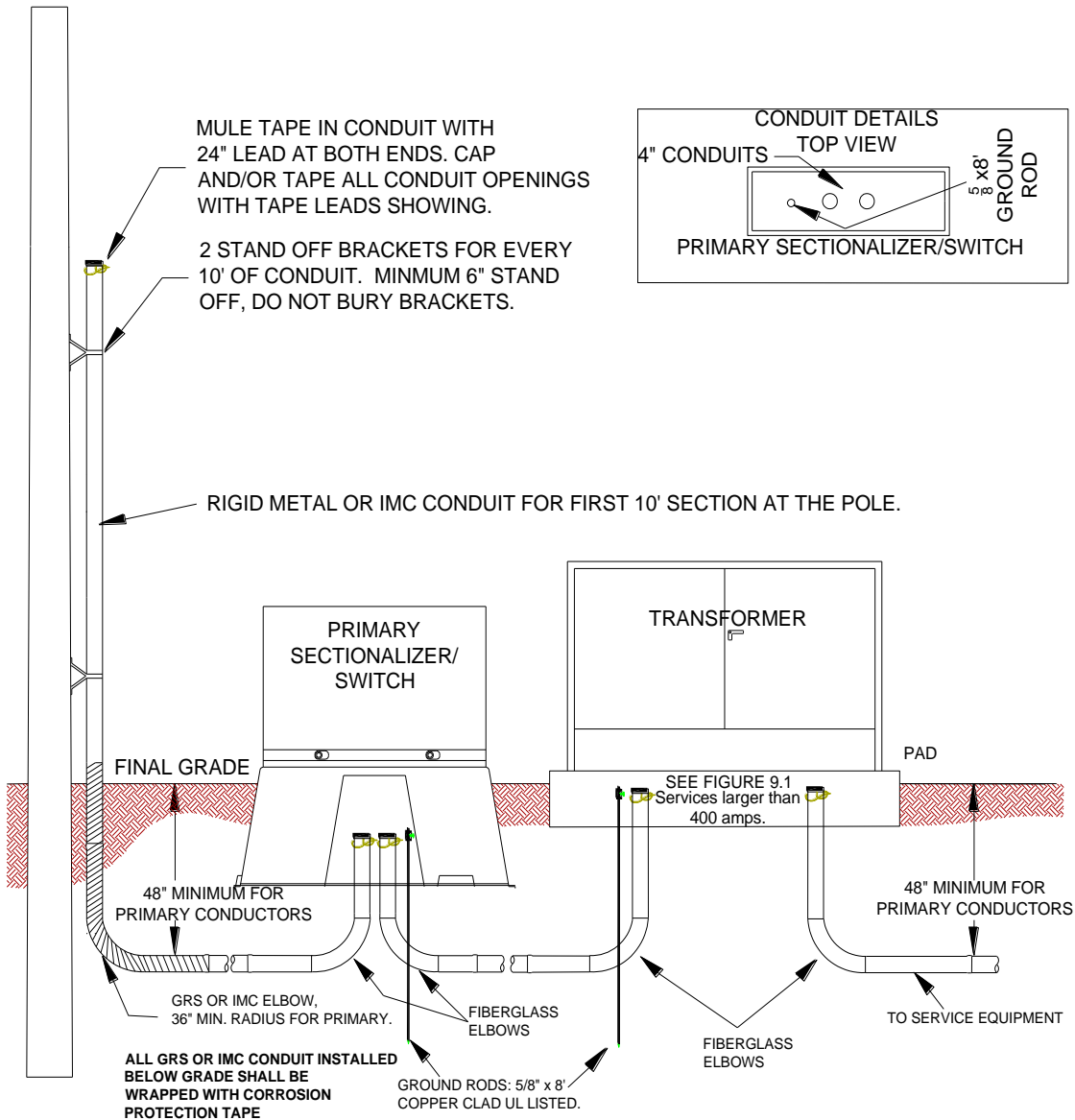
Figure 4.1 Underground Distribution
