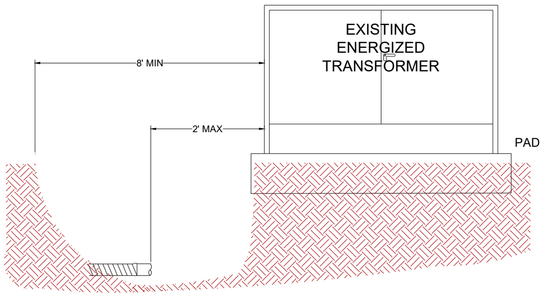
Figure 15.1.3 Connecting to a Transformer
