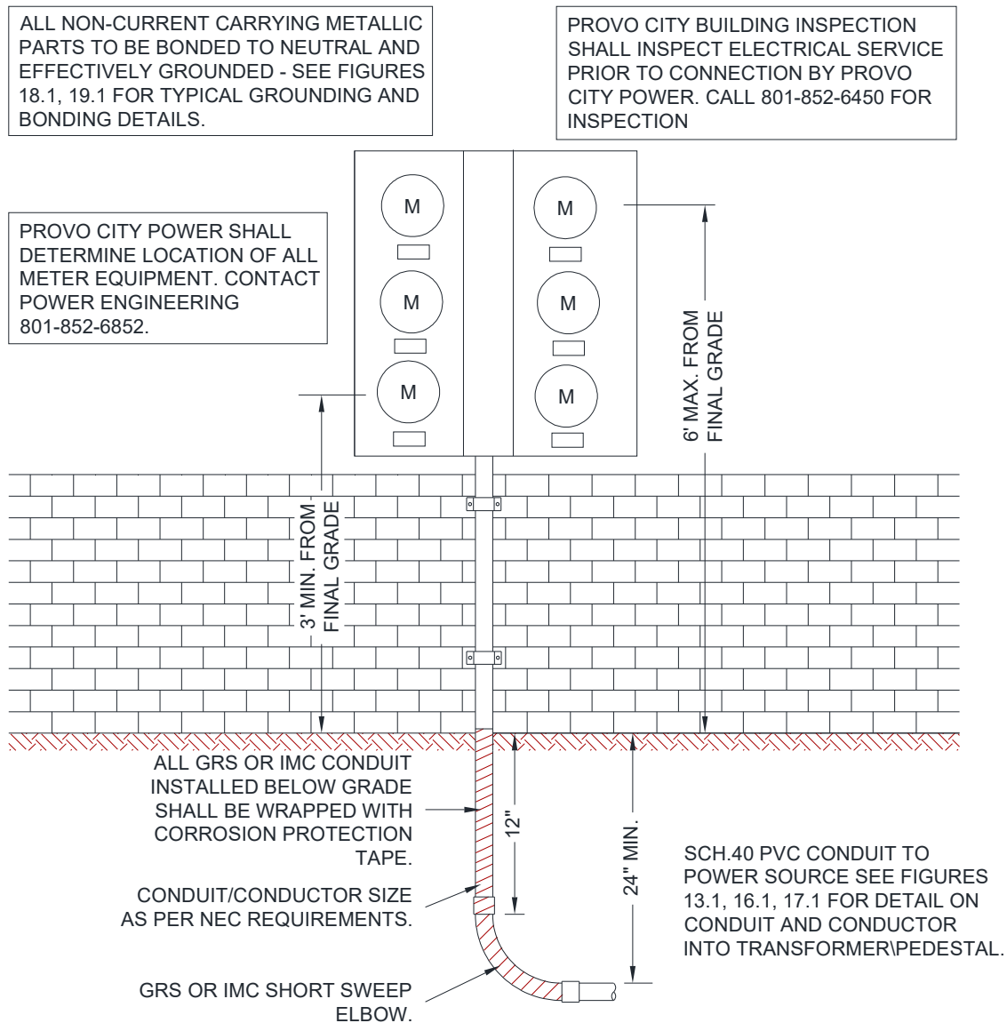
Figure 7.1 Multi-meter Installation
