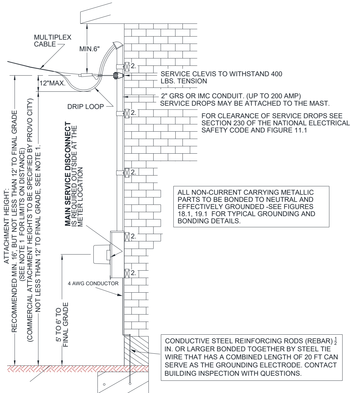
Figure 10.1 Under Eve Installation
