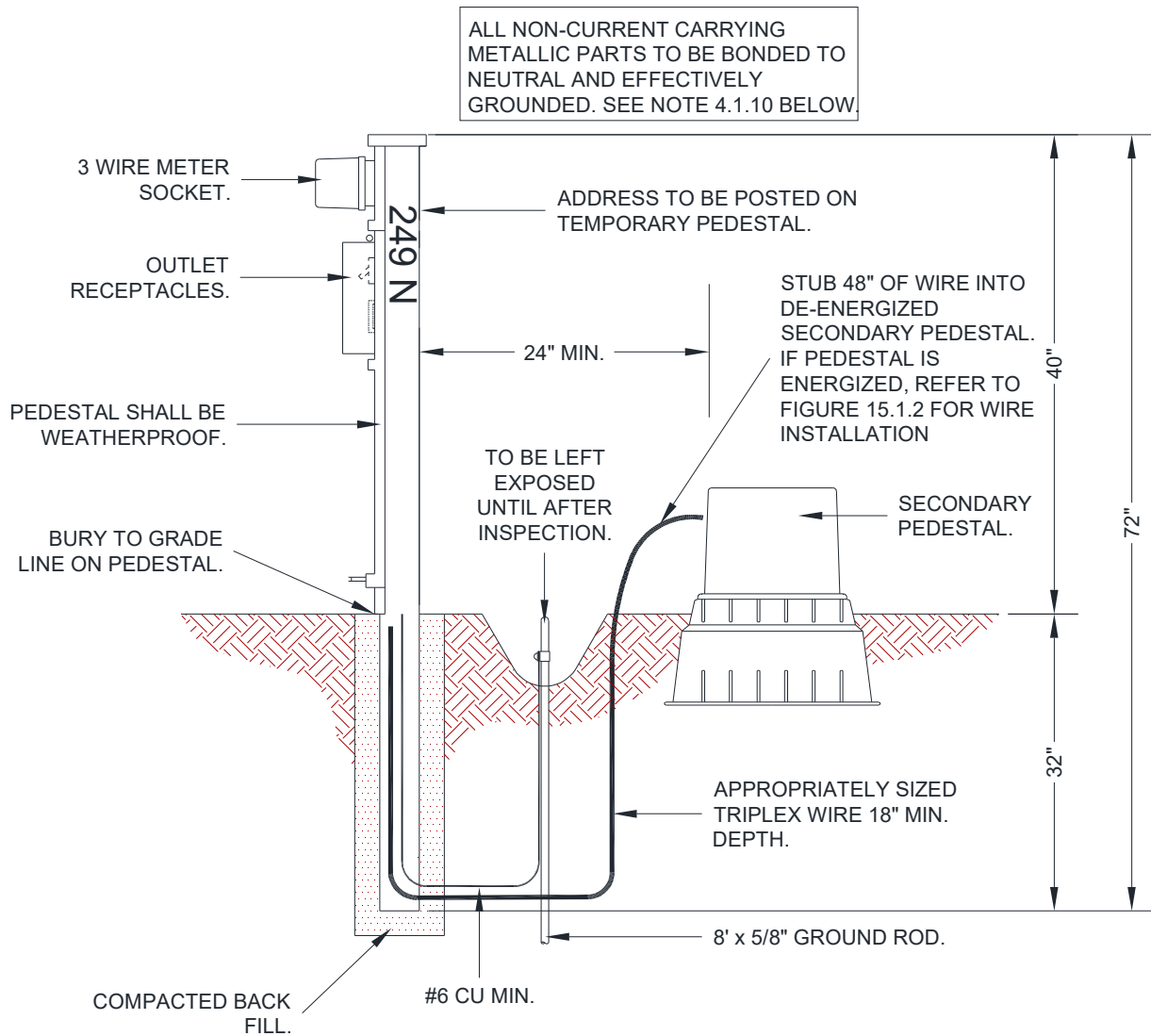
Figure 4.1 Meter Pedestal
