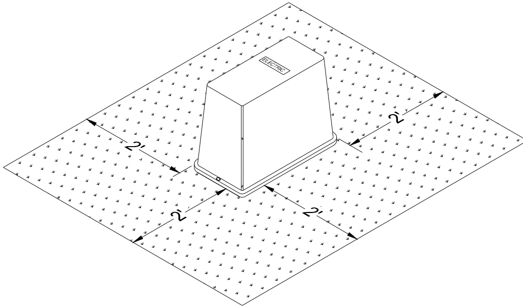
Figure 17.1 Secondary Pedestal (Typ. 12"x20" lid approx.)
