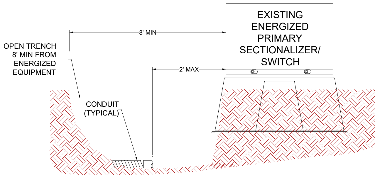
Figure 15.1.1 Connecting to a Sectionalizer
