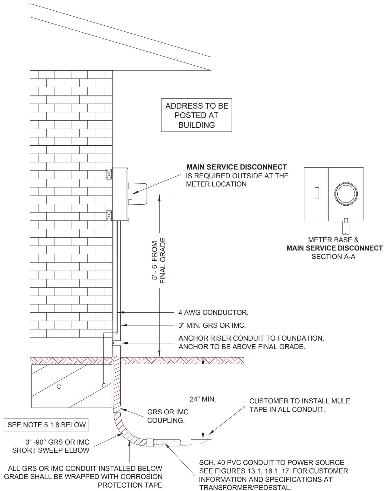
Figure 5.1 Underground Service Installation
