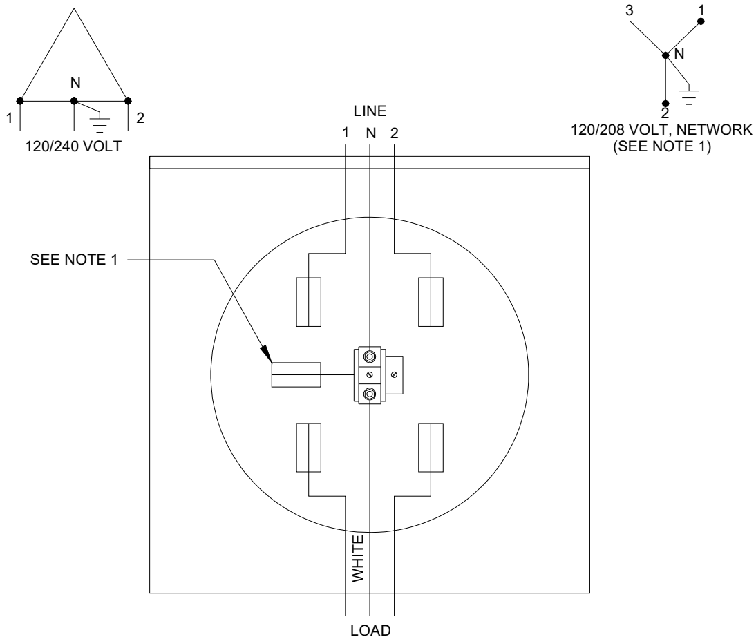
Figure 12.1 Meter Socket Wiring Diagram
