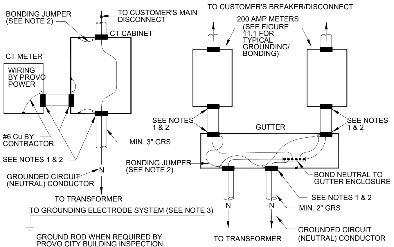
Figure 19.1 Typical CT Cabinet Grounding and Bonding
