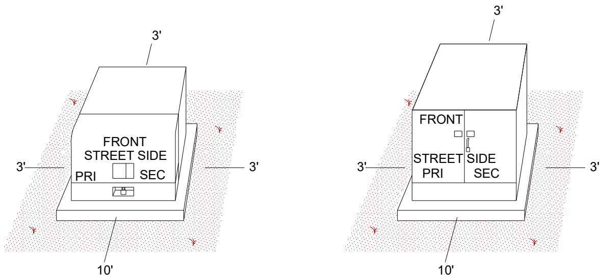
RESIDENTIAL SINGLE-PHASE TRANSFORMER PADMOUNTED EQUIPMENT
