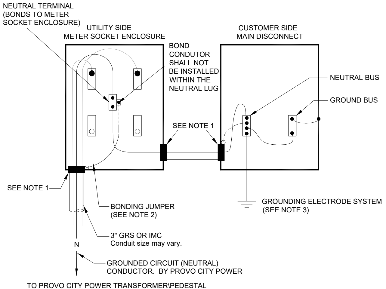
Figure 18.1 Typical Grounding and Bonding
