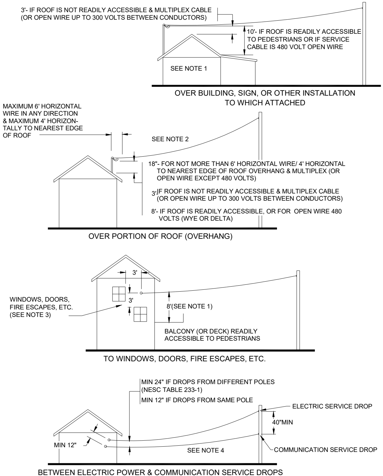
Figure 11.1 Clearances of 600 Volt Service Drops.
